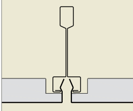
CLIP-IN
